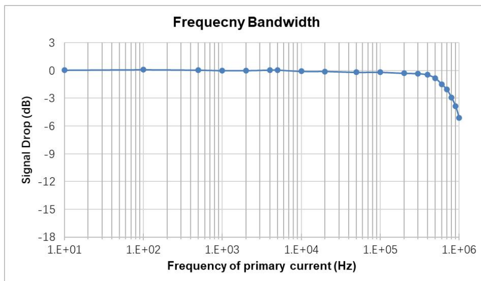
STK-600/F bandwidth
