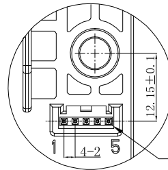
Detail-H 2:1
