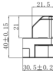
Detail-H 2:1
