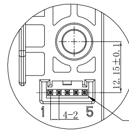
Detail-H 2:1
