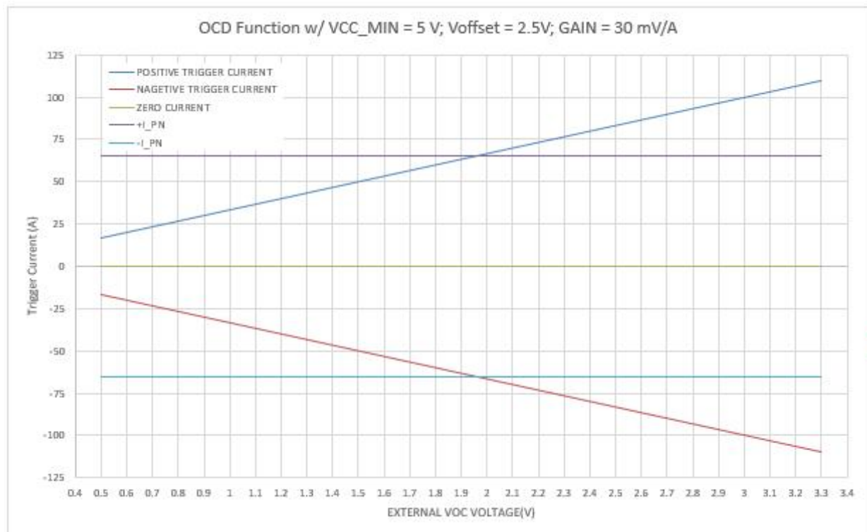
OCD function for STK-616T-65MAFB5
