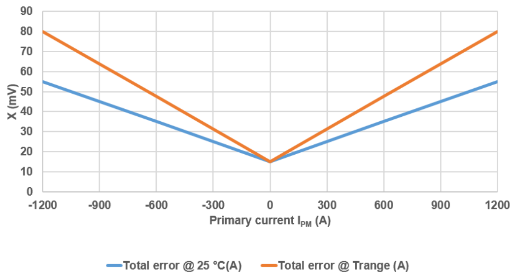
SHK-VBS-A3-S3: Overall accuracy X @ Vcc 5V (-40℃≤ Ta ≤125℃) absolute error
