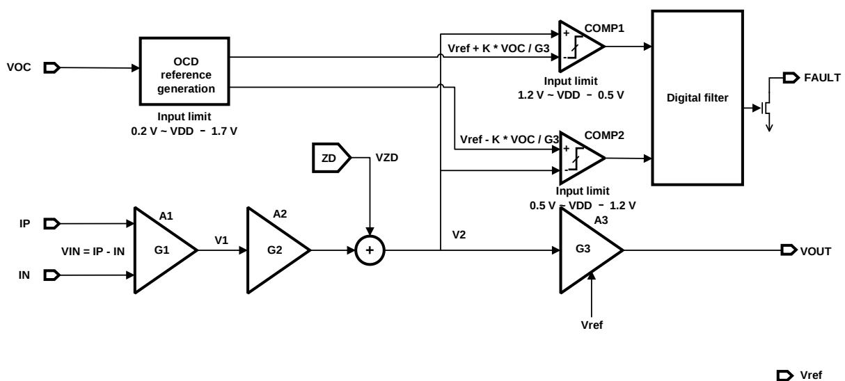
Figure 9 the functional block diagram for STK-626TMF on OCD function with conditions of V_{cc} = 5\text{ V} , V_{\text{off}} = 2.5\text{ V} , V_{\text{ref}} = 2.5\text{ V} .
