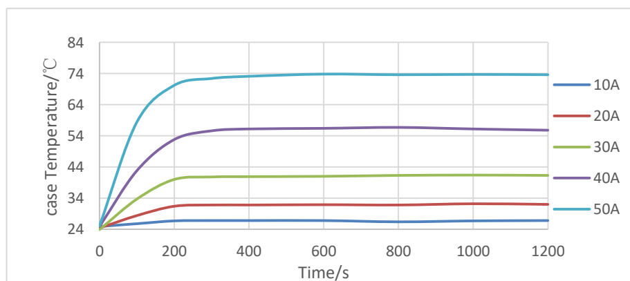
Figure 1. Relationship between STK-626TMF Case temperature and amount of input current.
