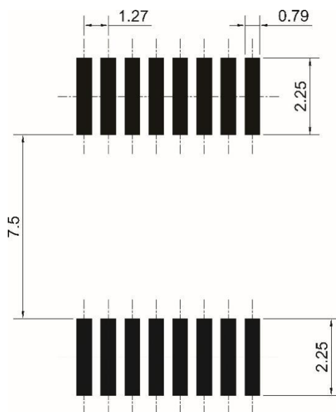
Figure 3. The recommended footprint of the SMT PCB layout for the STK-626TMF series products. The unit is mm.
