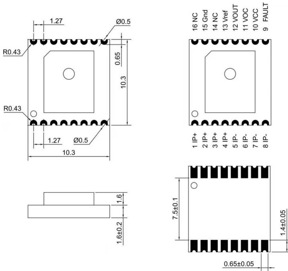
Figure 2. Dimensions of STK-626TMF series current sensors. The unit is mm.
