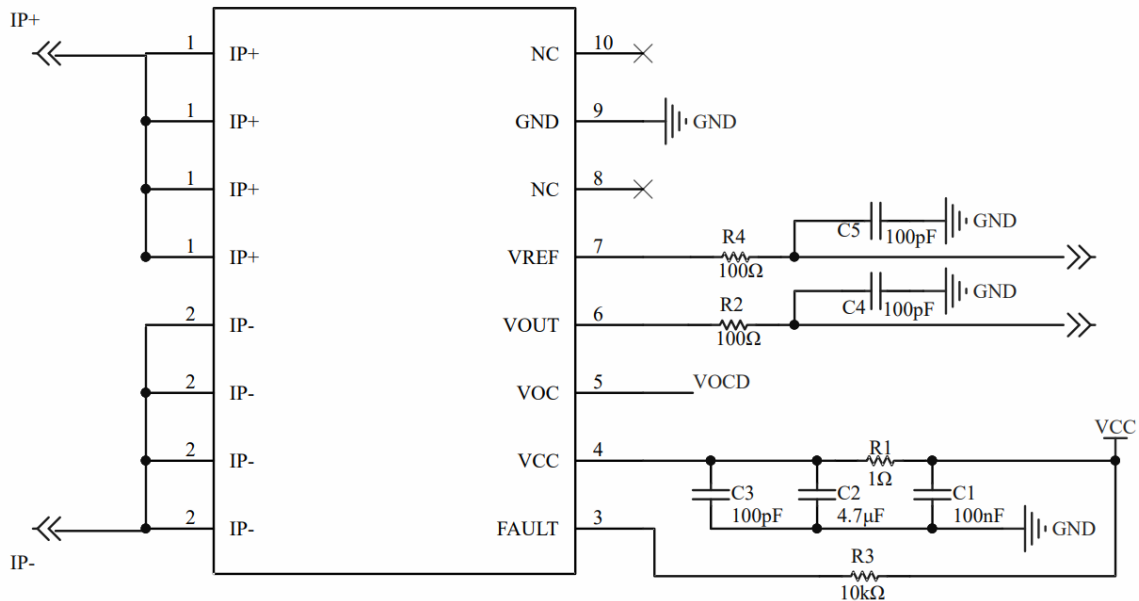
Figure 7. The reference application circuit for the STK-626TMF series products.
