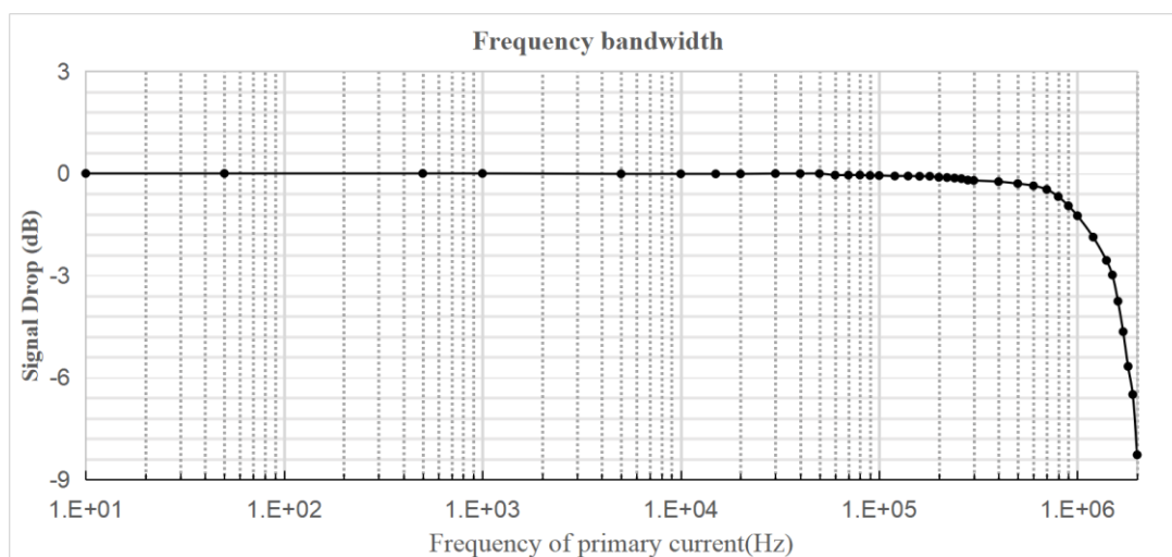
Figure 4. The frequency band width of the STK-626TMF series products. the upper limit of the -3 dB band width is 1 MHz.
