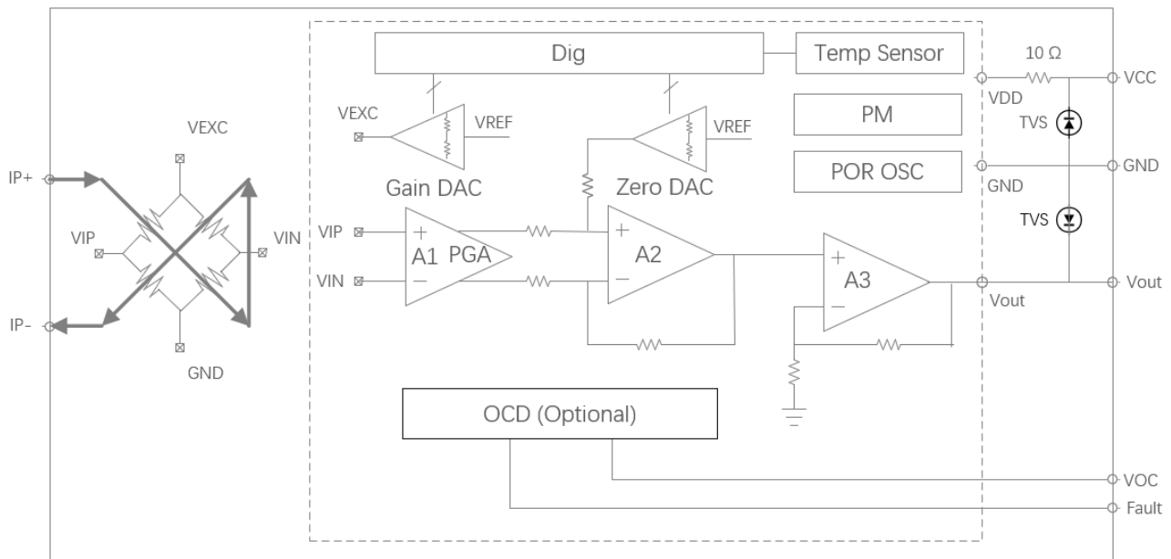
Figure 6. The functional block diagram for the STK-626TMF series products.
