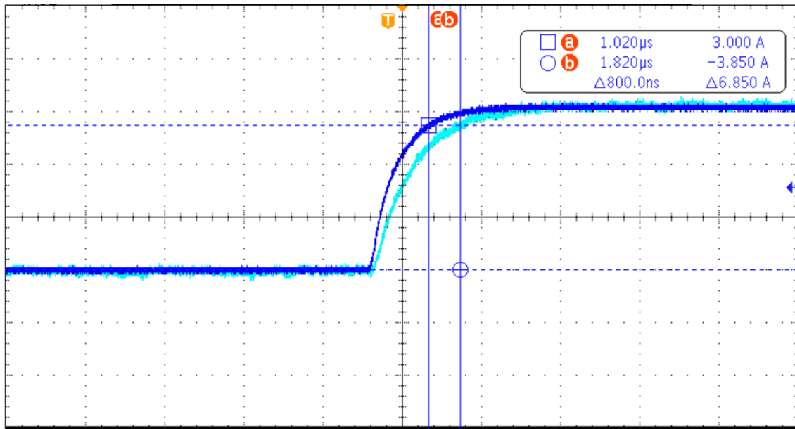
Figure 5. The typical frequency response of STK-616AM3 series current sensor. The response time from 90% of the primary current to 90% of the secondary output is 0.9 \mu s.
