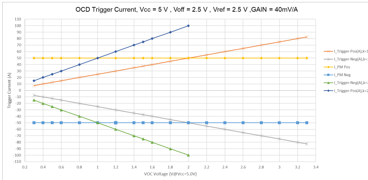
Figure 8 the relationship of trigger current and VOC setting for the STK-616T-50MFB5, with V_{cc} = 5\text{ V} . I_{\text{trigger\_pos}} represents the forward over-current protection trigger current. I_{\text{trigger\_neg}} represents the negative over-current protection trigger current. I_{\text{PN\_pos}} represents the forward primary nominal current. I_{\text{PN\_neg}} represents the negative primary nominal current. K is OCD coefficient, with typical
